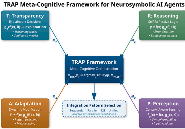
Fig. 7. The TRAP Meta-Cognitive Framework for Neurosymbolic AI Agents, illustrating integration of Transparency, Reasoning, Adaptation, and Perception components to orchestrate adaptive neuro-symbolic patterns.
